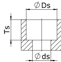
Countersunk hole
