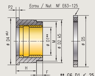
Ensemble / Assembly REF. 5355
